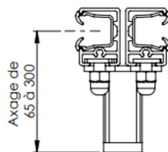
Equerre double
